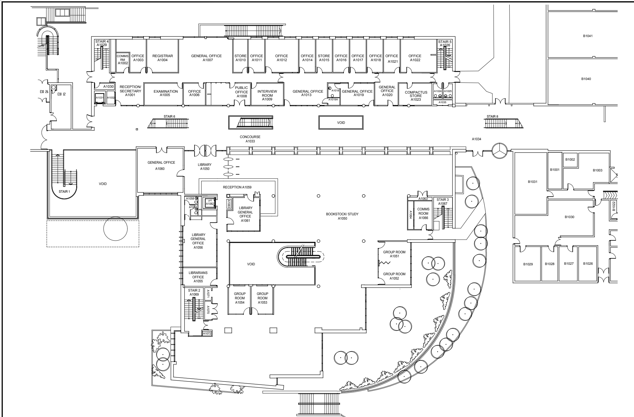
Block A - Library/ Admin Building
